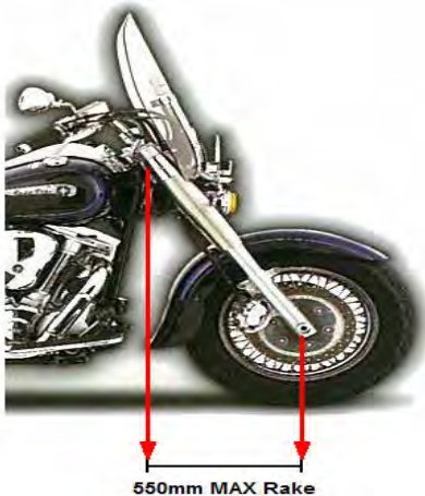
Motorbike Rake
